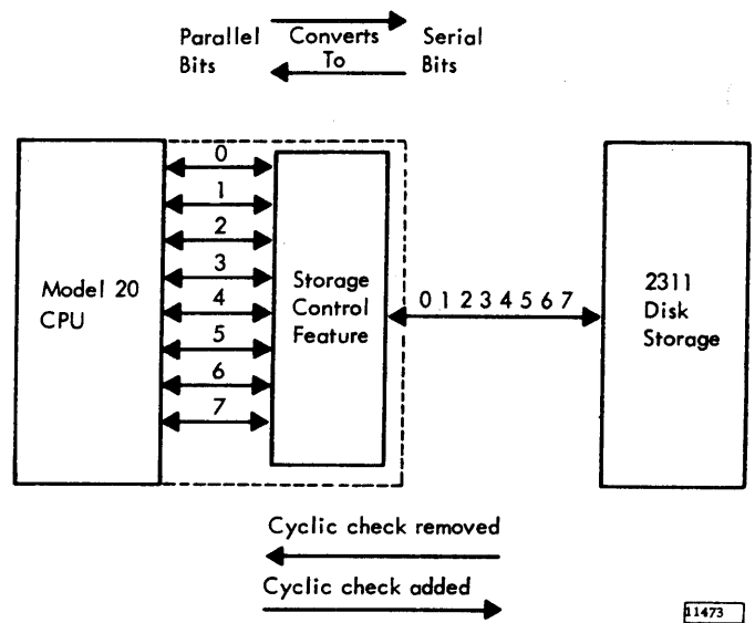
Figure 8. Data Transfer
