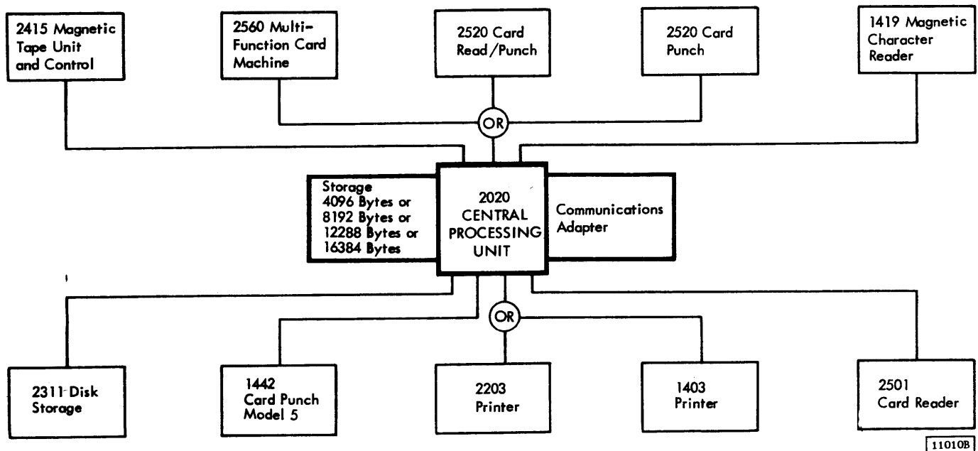
Figure 1. System/360 Model 20
