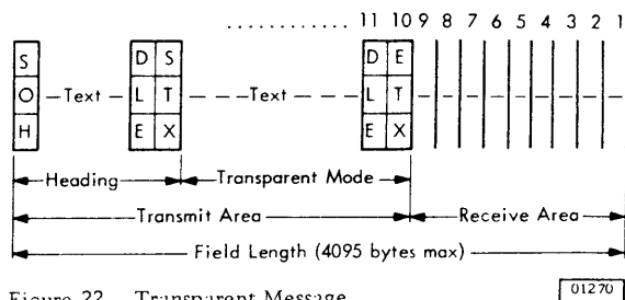
Figure 22. Transparent Message
