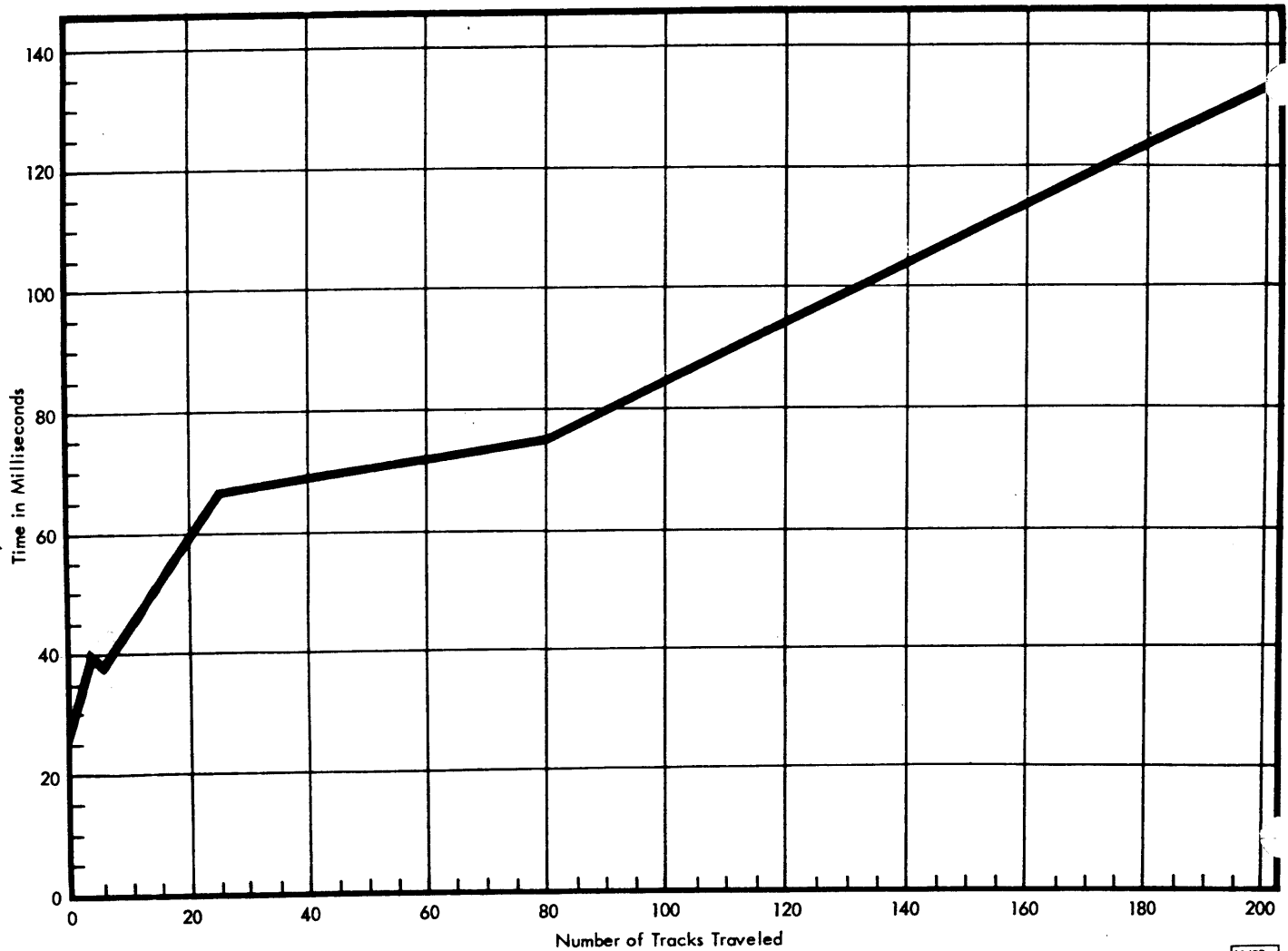
Figure 7. Access Time
