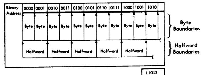
Figure 2. Integral Boundaries
